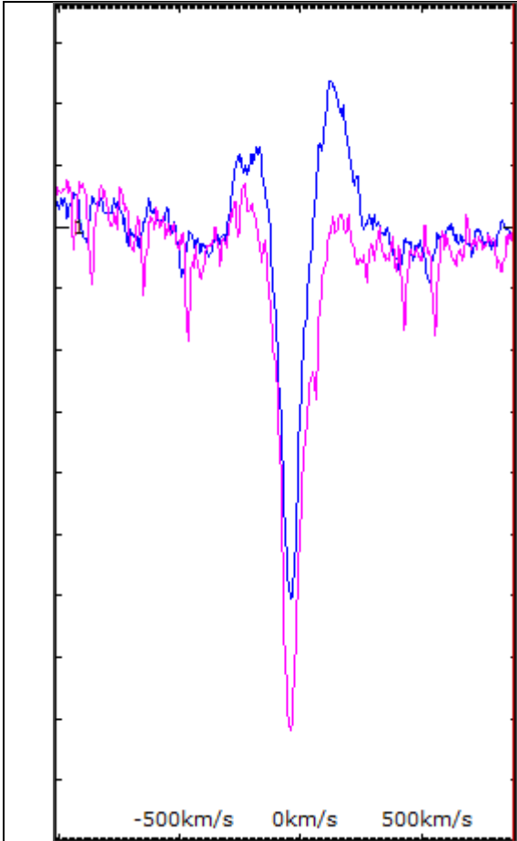
V2148 Cyg Increase of H-alpha emission
