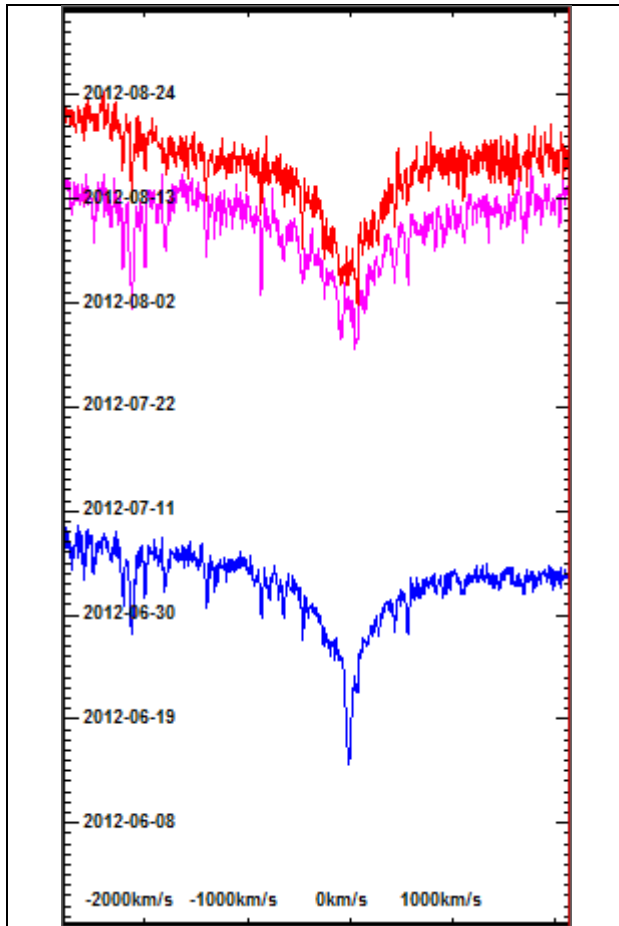
V2136 Cyg H-alpha wing emissions decreasing – 30/7/12- 30/11/11
