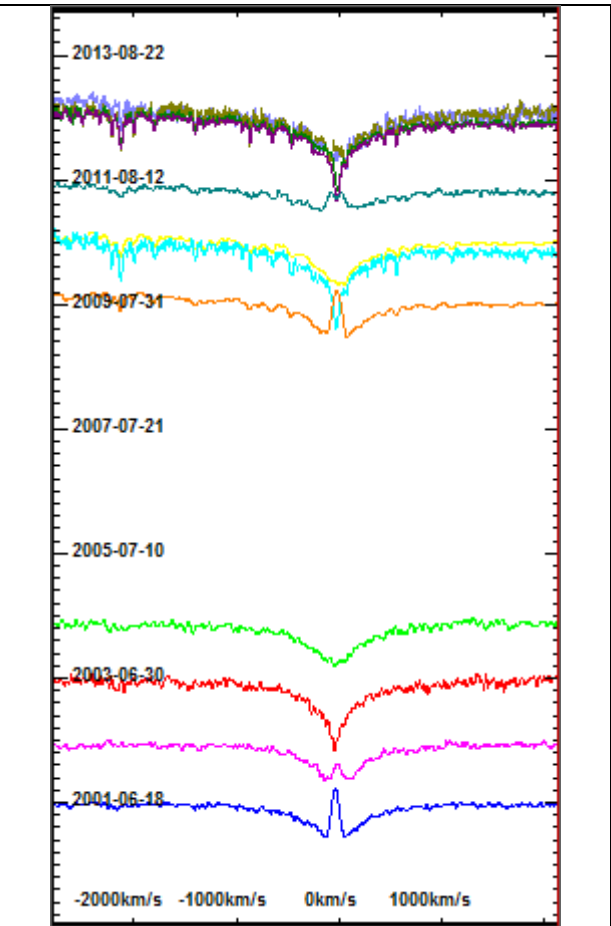
V2136 Cyg Time serie from 2002 – decrease of emission
