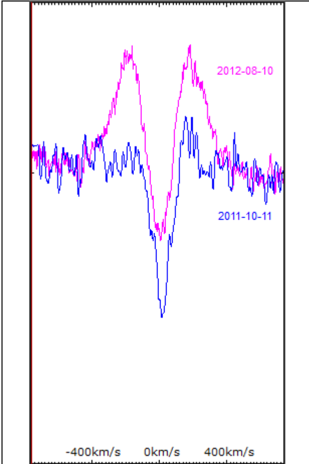
V787 Cas Stronger H-alpha line
